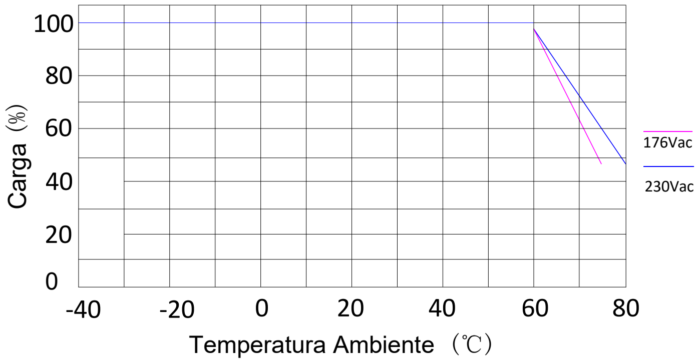
CURVA DE DERATING
